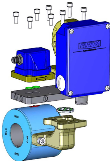
V- and M- series on FA pipe section
