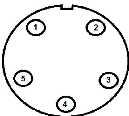
M9 - 5 pin
